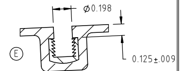
SECTION A-A SCALE 1:1 ALL 10-24 INSERTS
